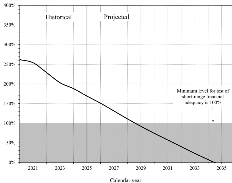
Figure II.D1.— OASI and DI Combined Trust Fund Ratio, 2020-2036
