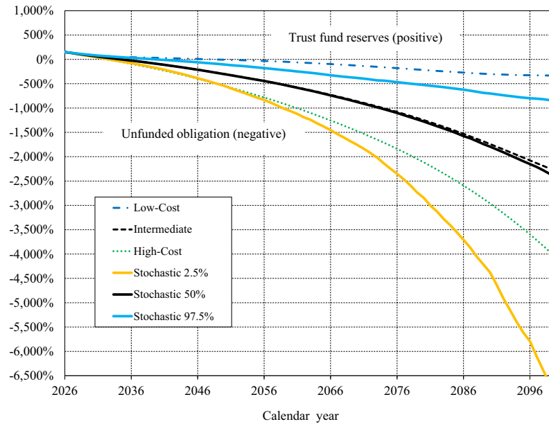
Figure VI.E4.—OASI and DI Combined Trust Fund (Unfunded Obligation) Ratios: Comparison of Stochastic to Low-Cost, Intermediate, and High-Cost Alternative Scenarios a
